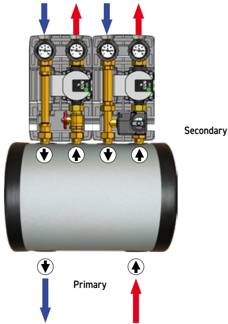
Schematics: buffer tank installed horizontally
