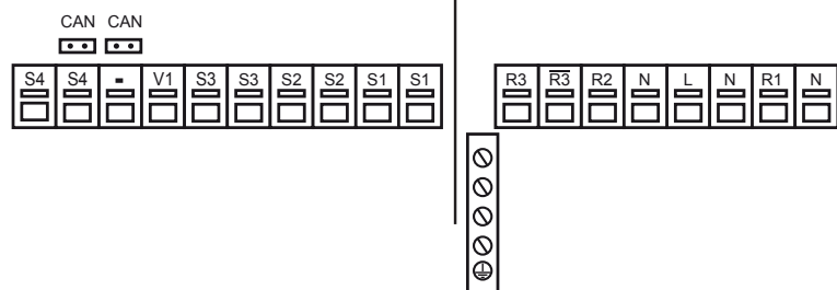
Pict 3: Connection terminal of the climatic controller
