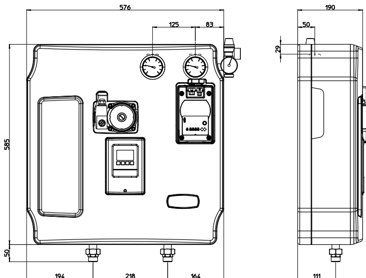
Figure 3: overall measurements and main wheelbases of the unit.
